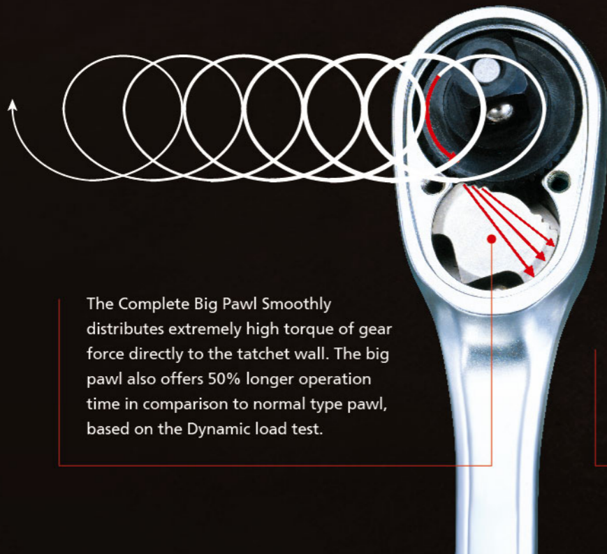
KH2400 RATCHET
