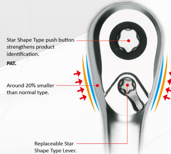
KH2800 RATCHET
